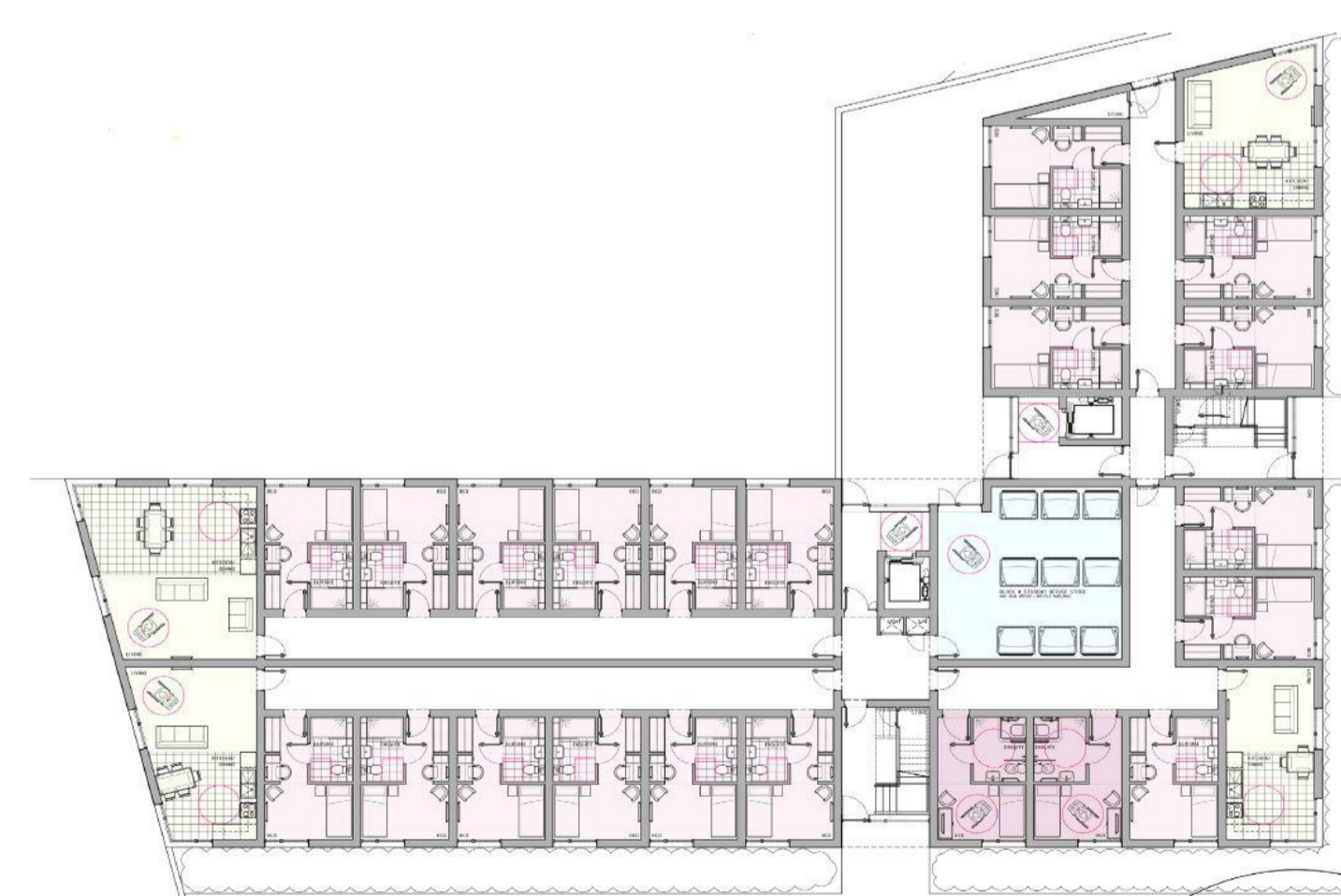
Typical Block A Floorplan
