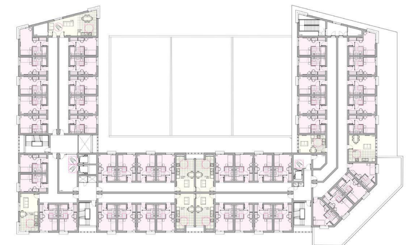
Typical Block B Floorplan
